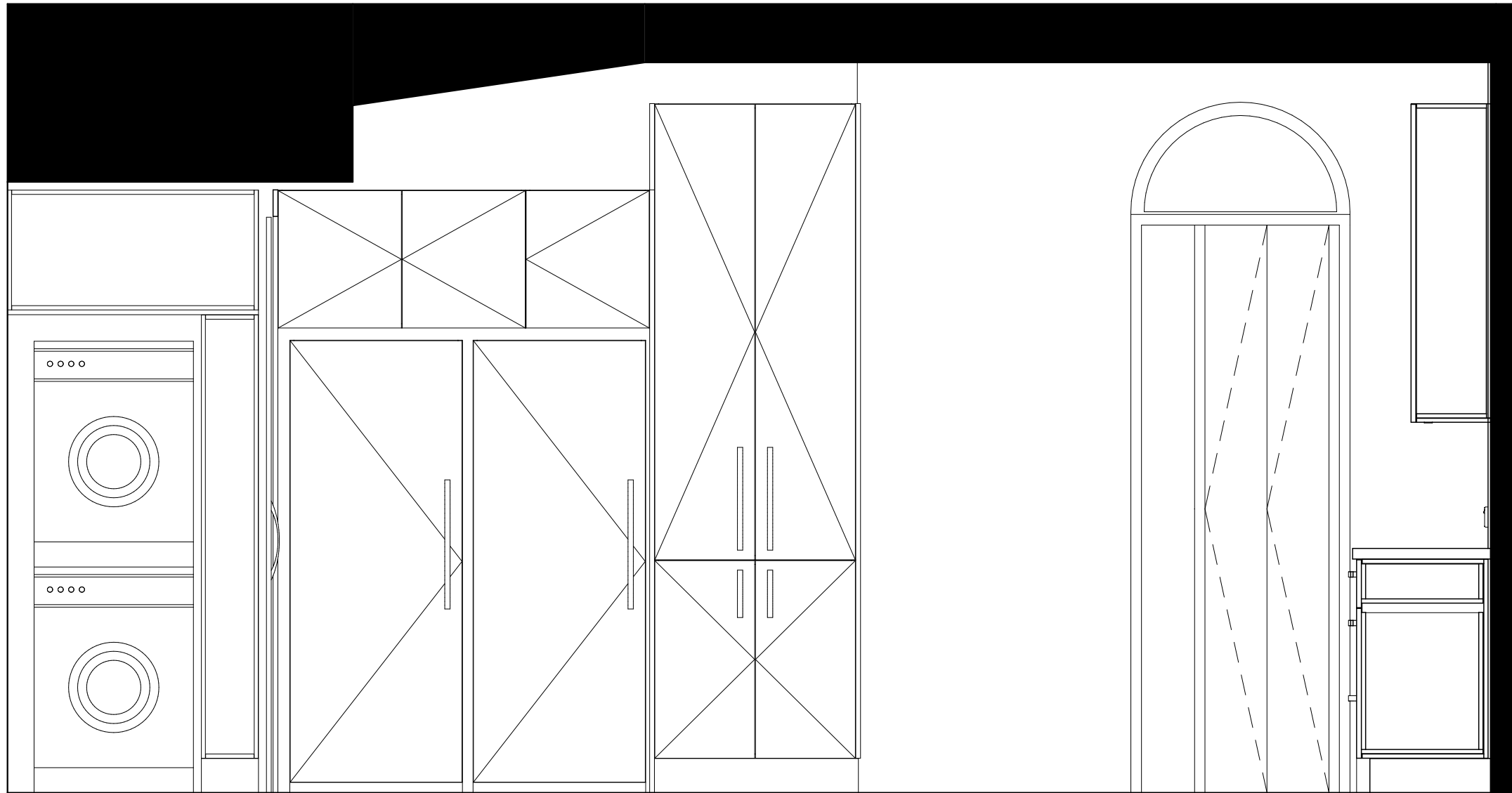
C - SECTION, 1:20
